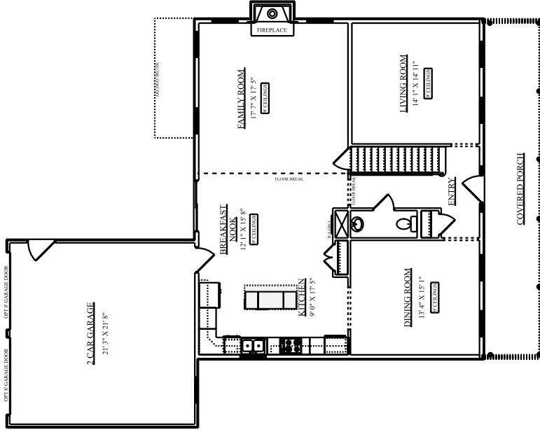
MAIN LEVEL 1383 SQ FT
