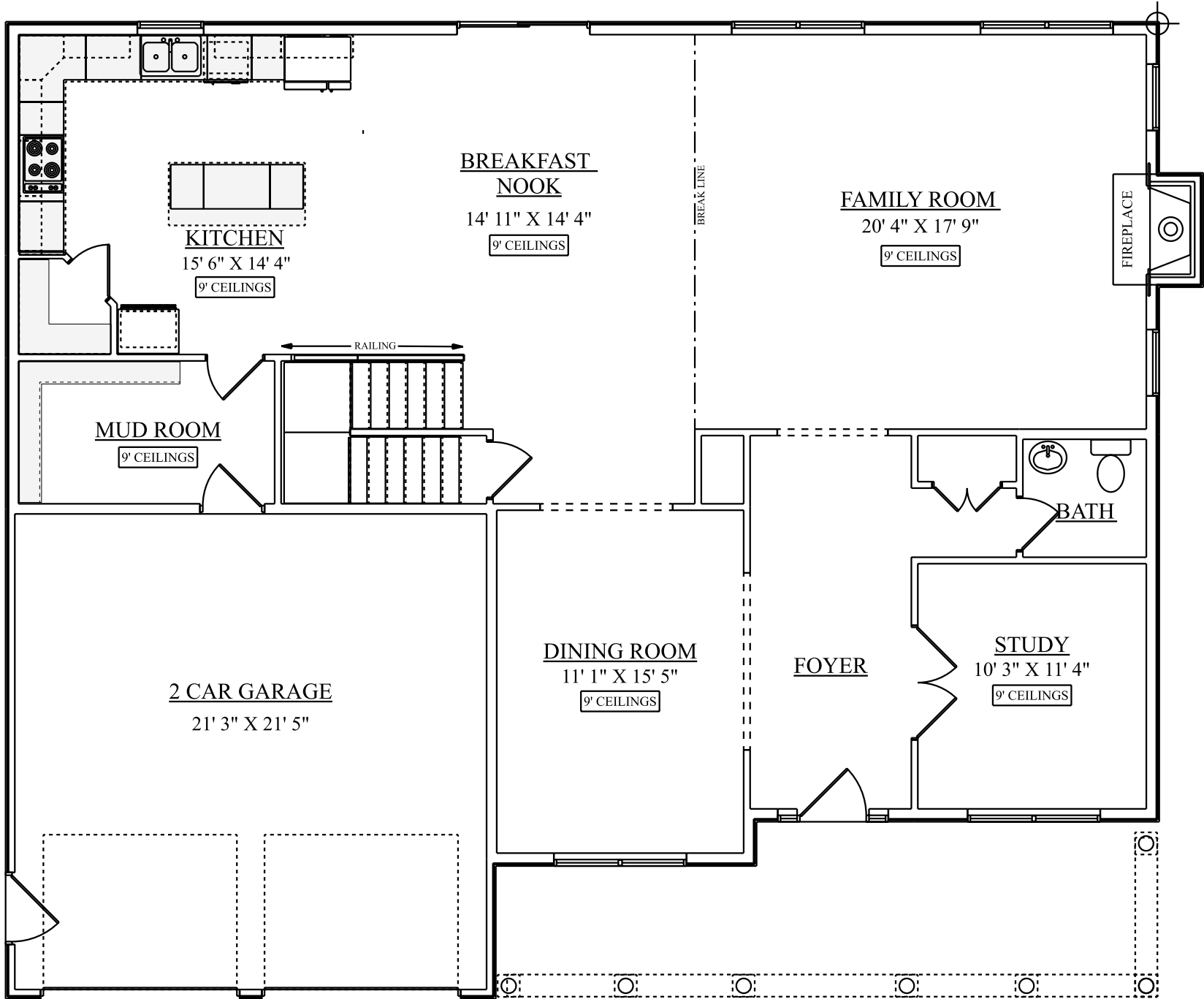
1ST FLOOR 1615 SQ FT
