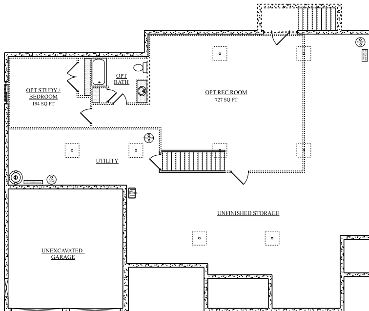
LOWER LEVEL 2502 SQ FT
