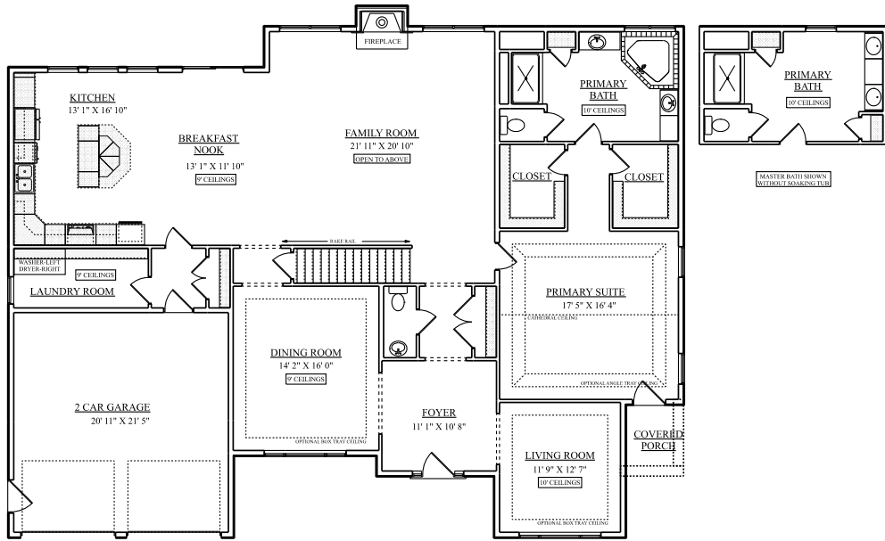
MAIN LEVEL 2470 SQ FT
