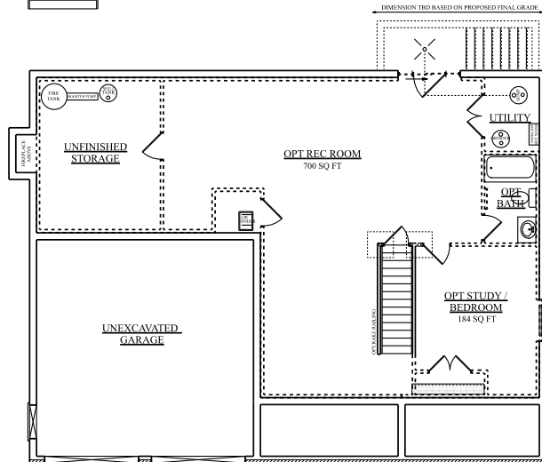
LOWER LEVEL 1281 SQ FT
