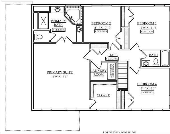
UPPER LEVEL 1312 SQ FT
